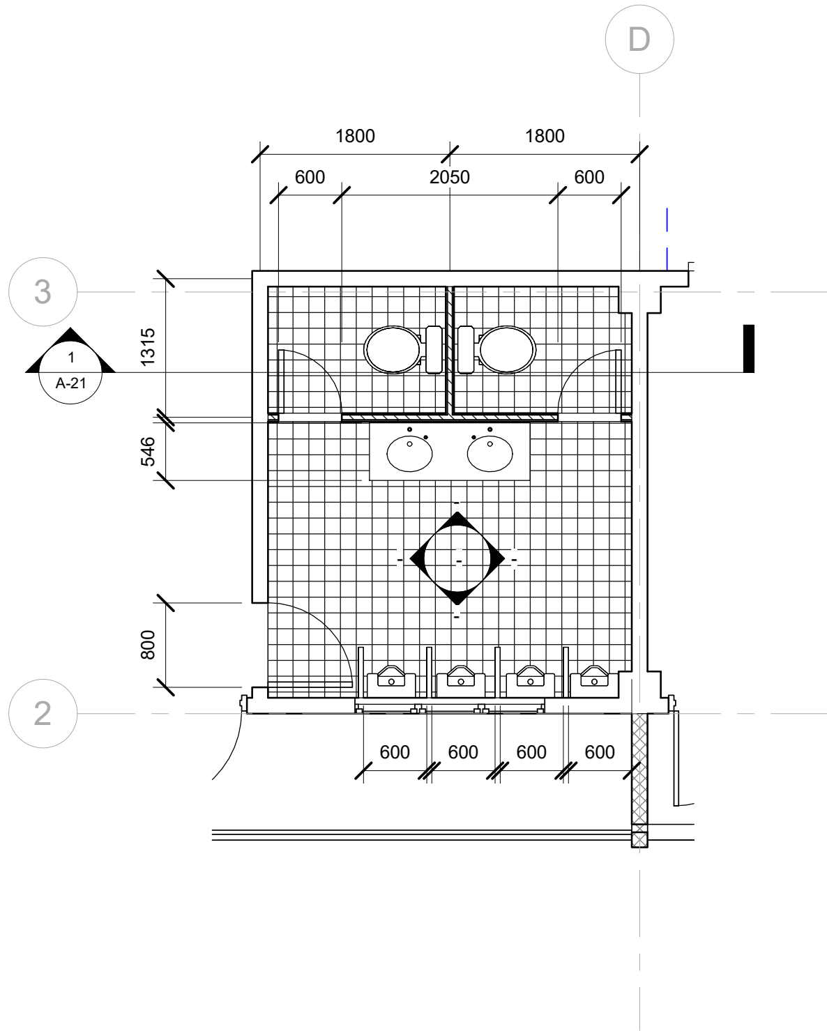
1 MALE CR PLAN
