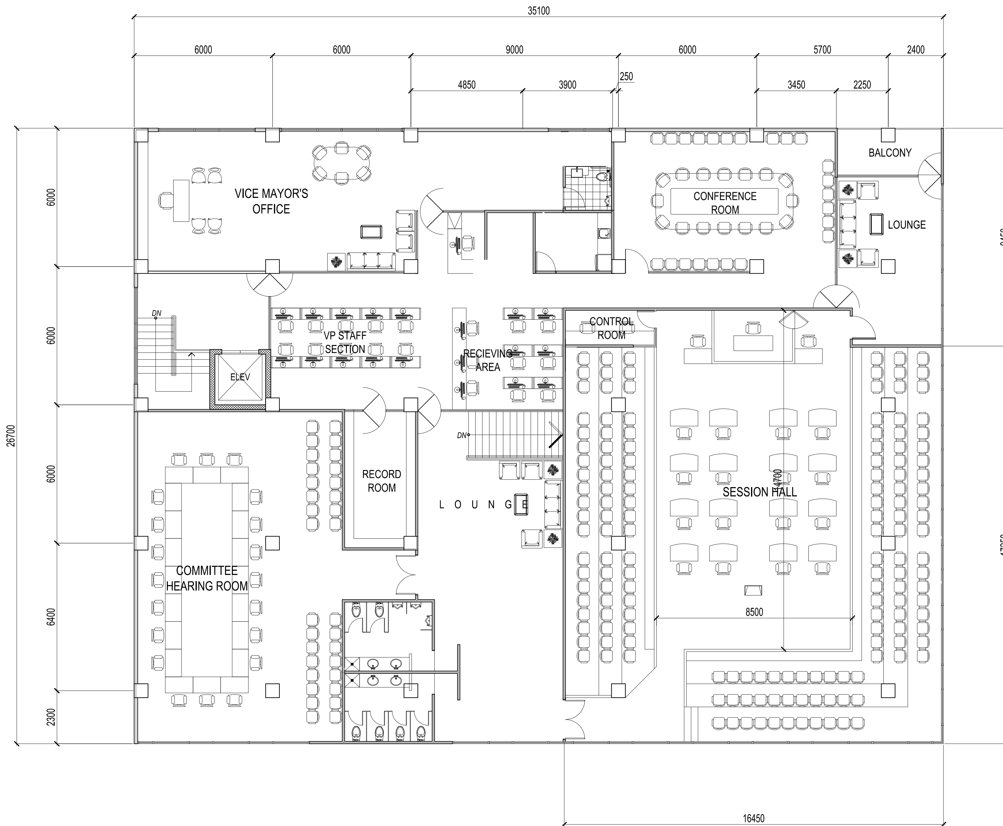
1 THIRD FLOOR PLAN A 5 SCALE: 1:100M
